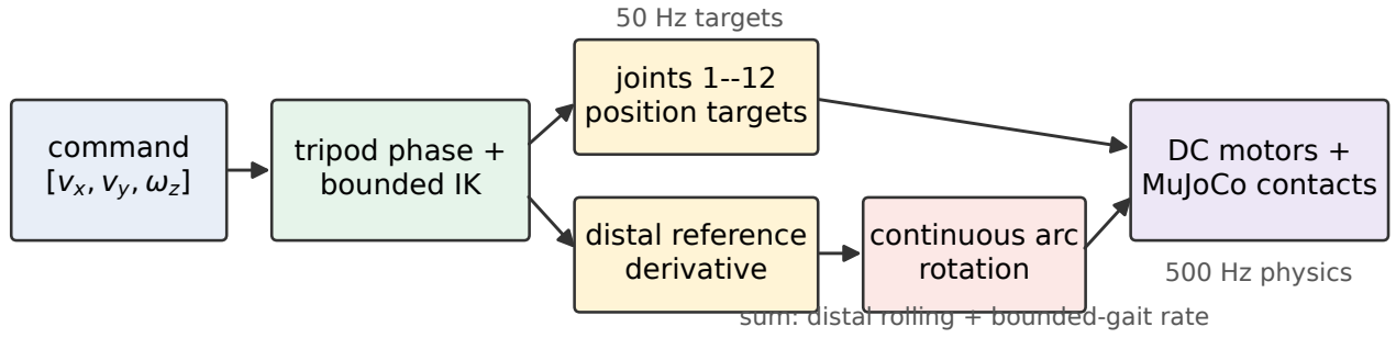
Fig. 3. Control paths. Joints 1–12 track the bounded tripod reference in position mode while joints 13–18 run in velocity mode and add continuous arc rotation to the differentiated reference, so walking and rotation are commanded at the same instant. The controller outputs 12 position targets and six velocity targets; no learned policy is used in the reported experiments.
