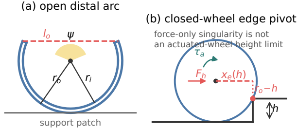
Fig. 2. Contact geometry of one distal link. (a) The open sector: outer and inner radii r_o, r_i , opening angle \psi and opening chord l_o , with the lowest patch acting as the support point during walking. (b) The closed-wheel pivot used to separate horizontal axle force F_h from applied axle torque \tau_a . A force-only push becomes singular as h \rightarrow r_o , but this is not a universal height bound for an actuated wheel.
