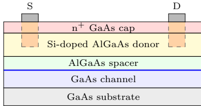
a) After ohmic contact formation
