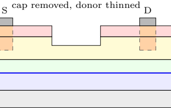
(b) Gate recess etched
