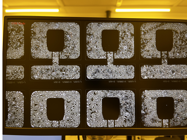
Figure 3.4: Ohmic contacts under x5 microscopy following lift-off.
