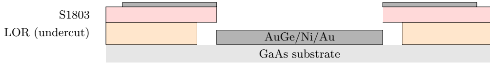
Figure 3.2: Dual-layer LOR/S1803 resist stack after development showing the wider LOR opening that creates an undercut for clean metal lift-off.
