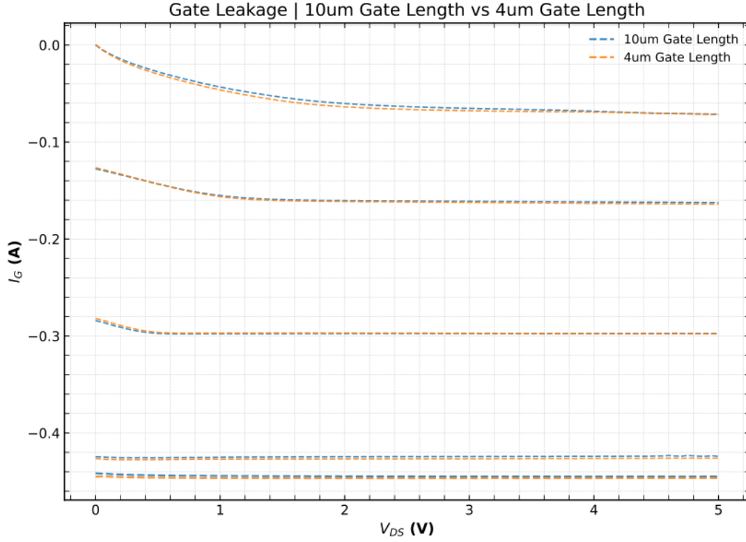
Figure 4.3: Measured gate leakage characteristics of the fabricated depletion-mode GaAs/AlGaAs HEMTs. Curves show averaged responses for each gate length, with comparison between the shortest and longest gate geometries highlighted.
