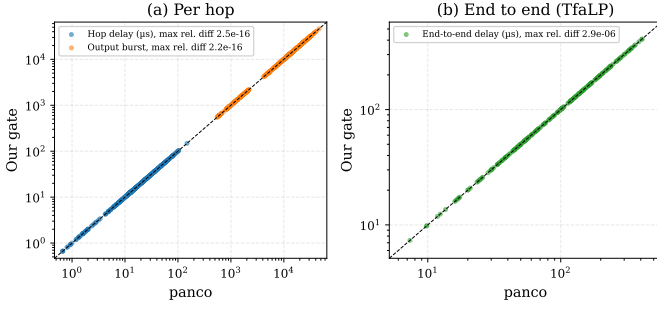
Fig. 2. Bounds of our gate against panco [6], per hop (1,119 values) and end to end (242 values, TfaLP).
