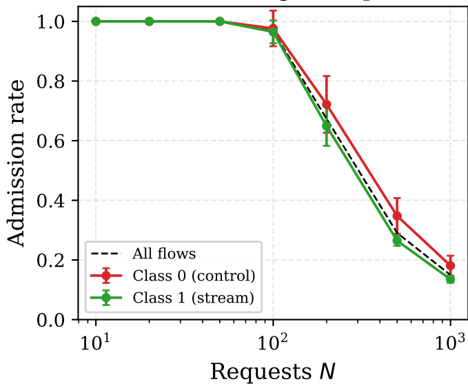
2 core \times 4 edge (56 ports)
