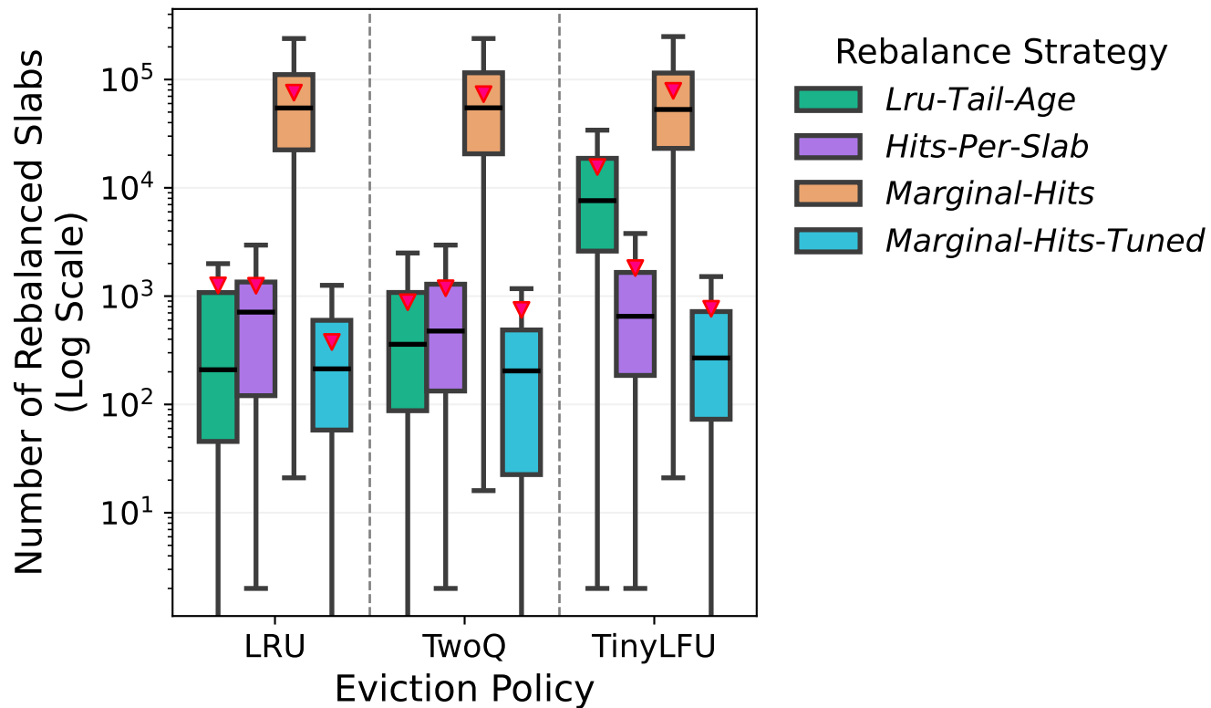
b. Twitter traces, large cache size
