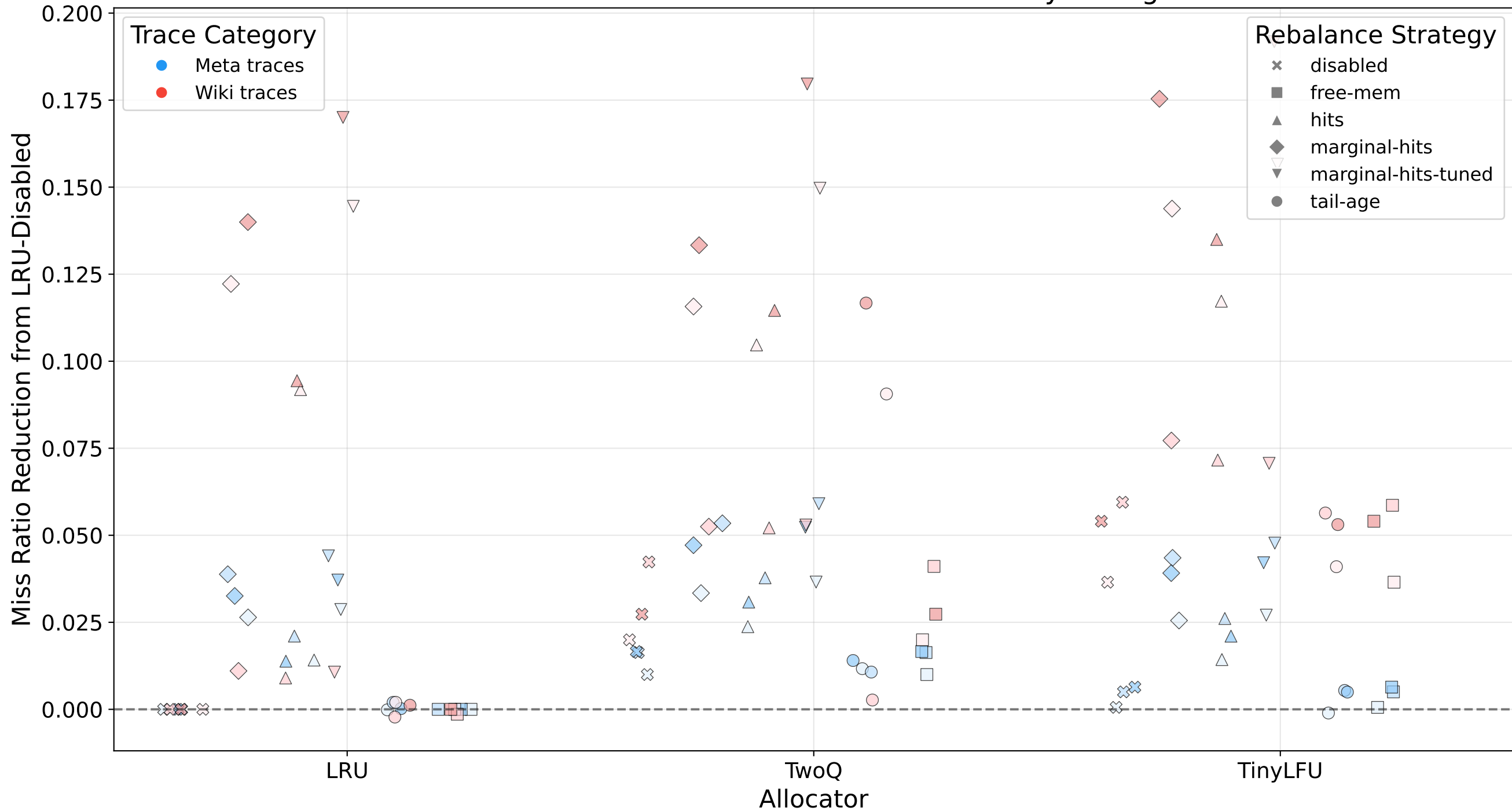
CDN Cache Performance: Miss Ratio Reduction by Configuration
