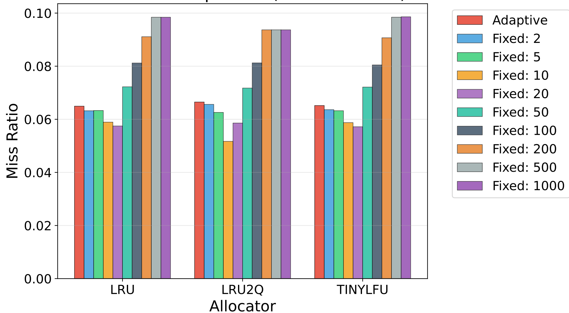
Threshold Comparison (WSR = 0.0100)
