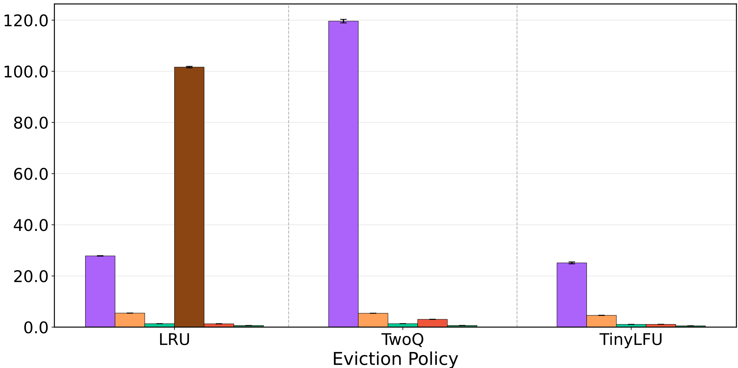
Rebalancing CPU Cycles Relative to Request Serving CPU Cycles (%)
