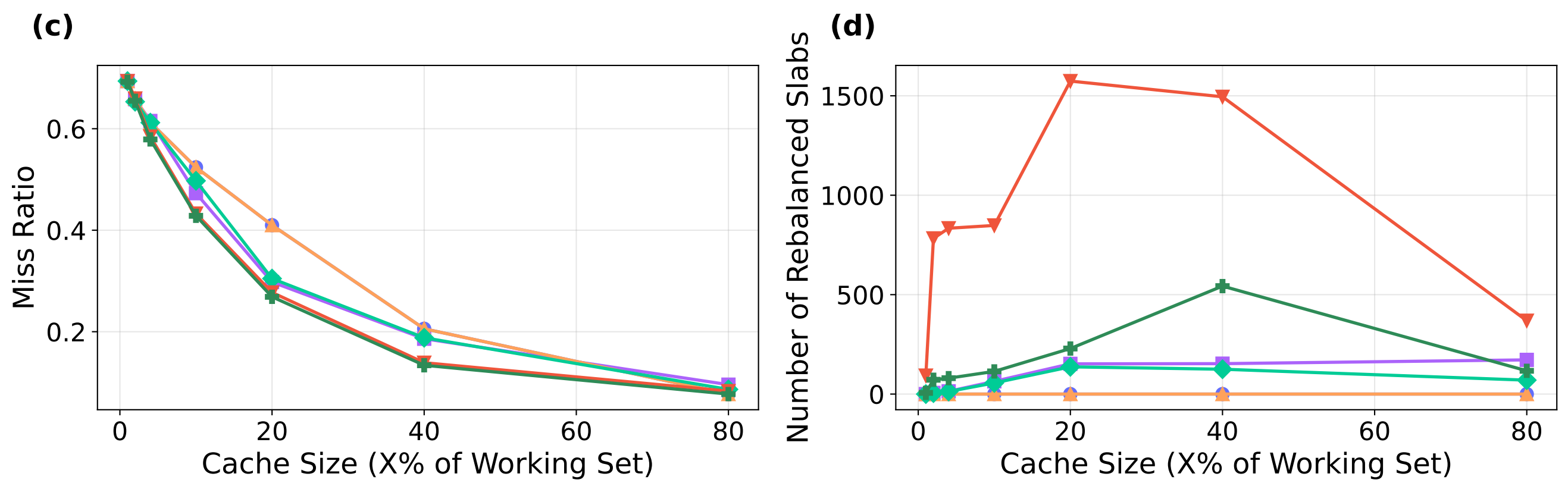
TwoQ
