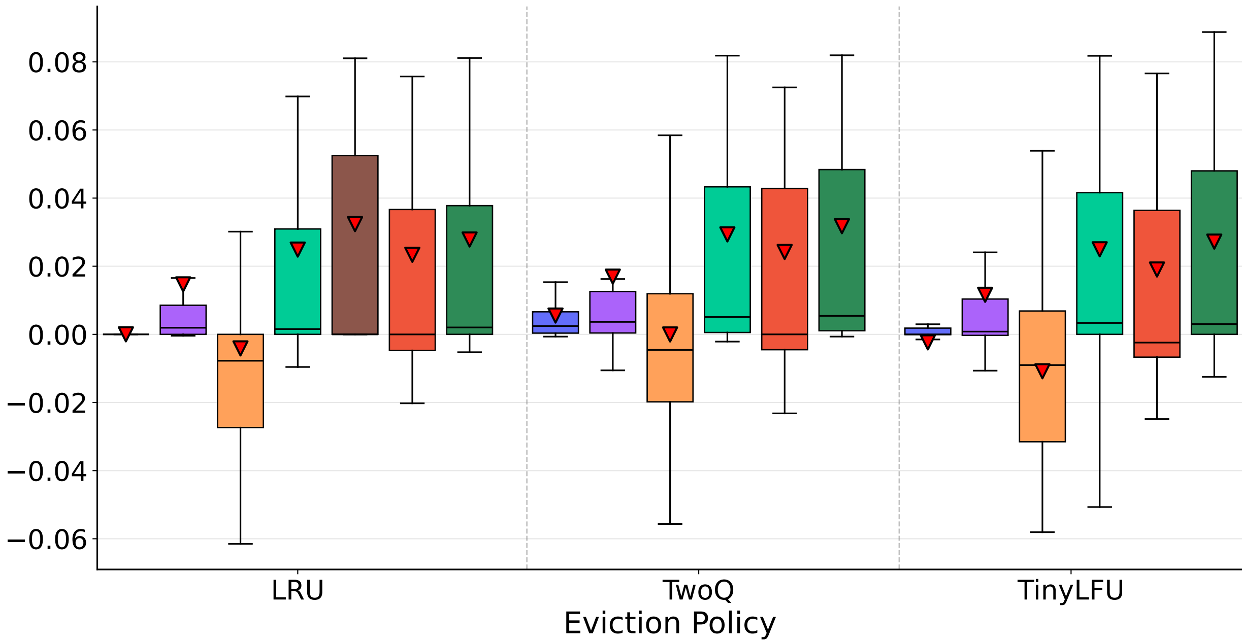
Miss Ratio Reduction over LRU + disabled
