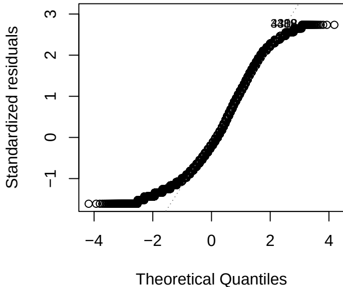
Q-Q Residuals
