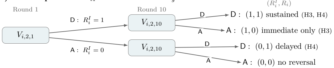
Figure 5: Decision tree for assignment and reversal. Each pool is assigned one value of T_g ; the primary analysis follows participants with A_{i1} = 1 .
