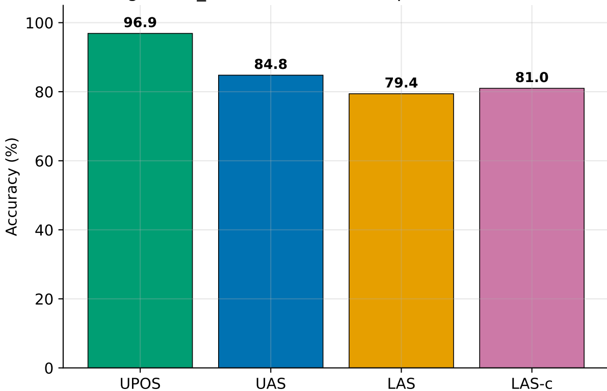
Parsing vs UD_French-GSD (n=416 phrases, 9108 tokens)
