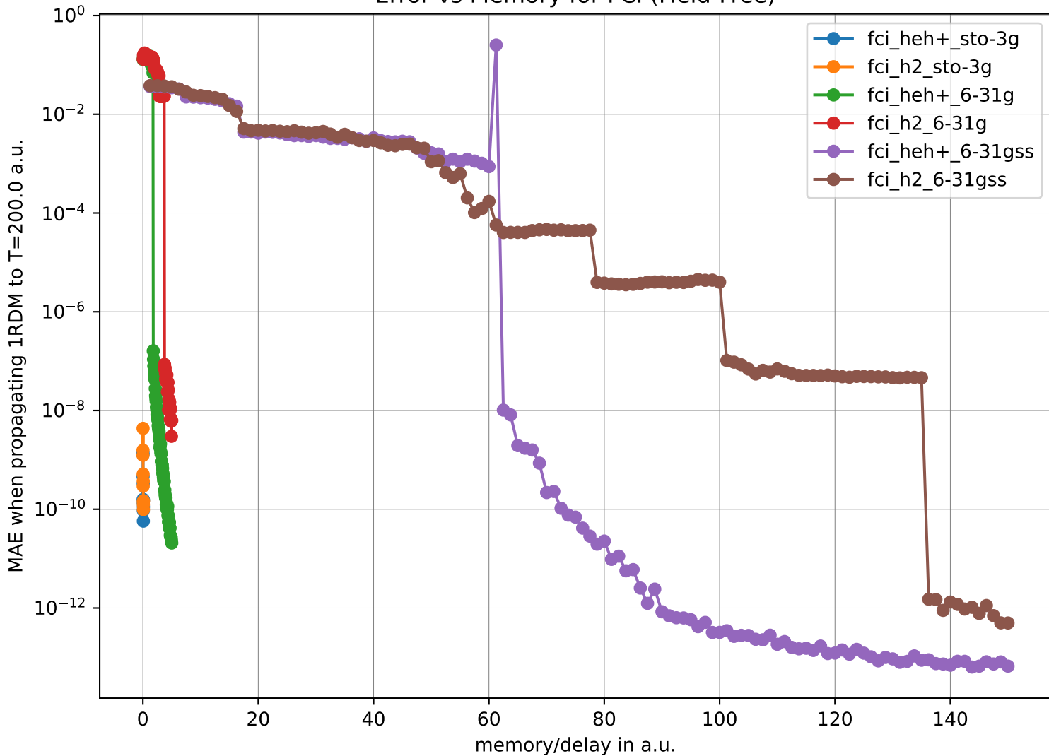
Error vs Memory for FCI (Field-Free)
