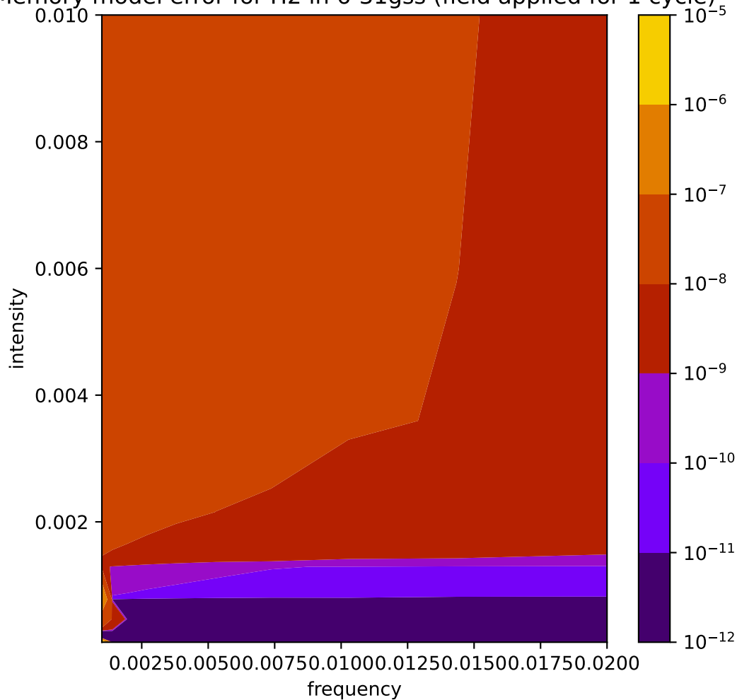
Memory model error for H2 in 6-31gss (field applied for 1 cycle)
