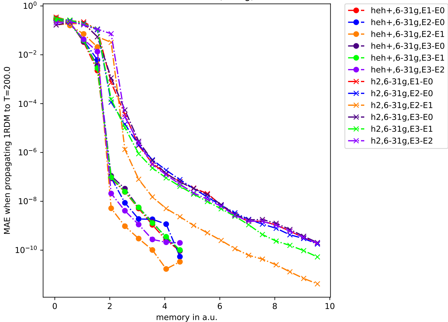
FCI Field-On Results (6-31g)
