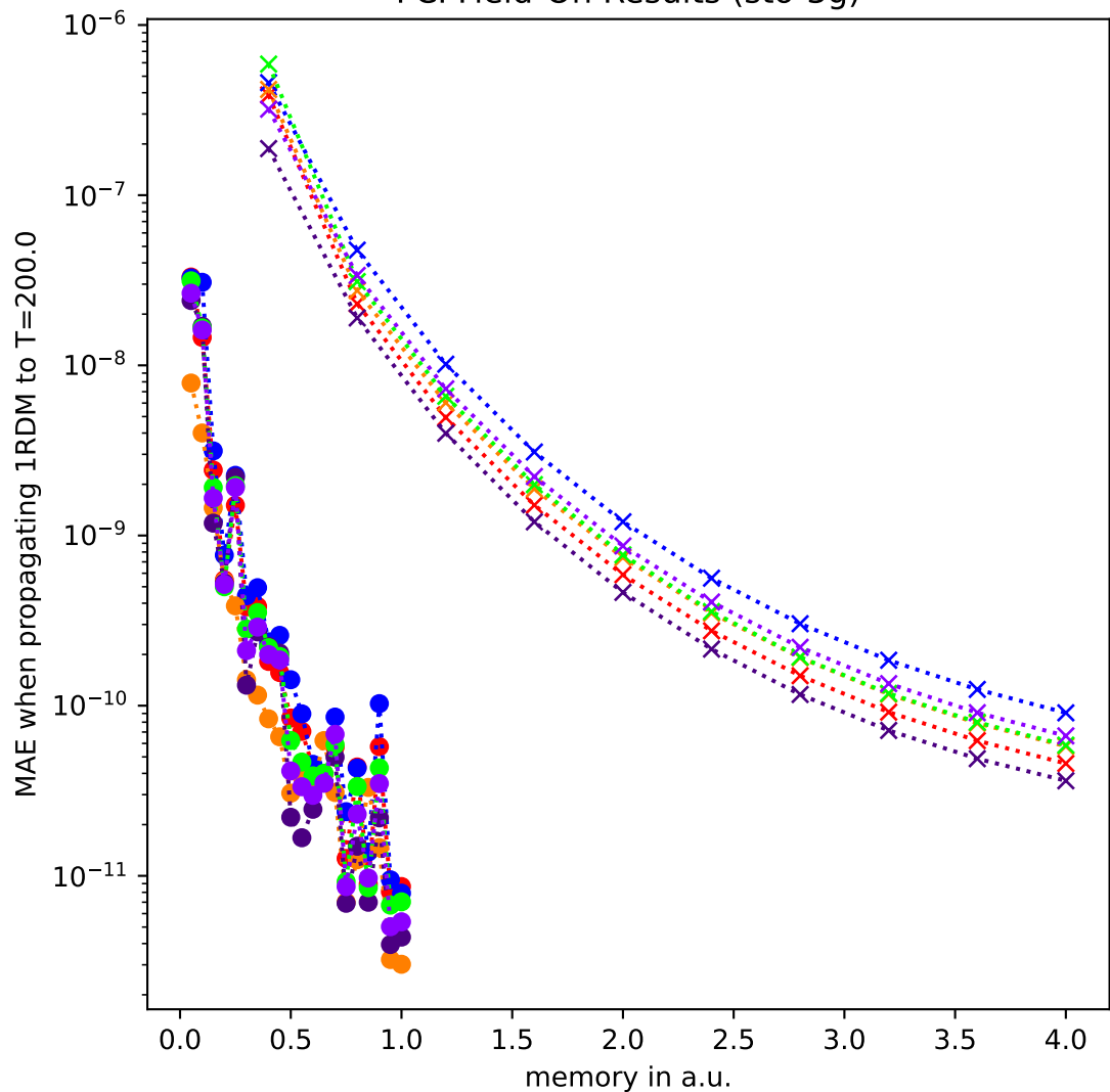
FCI Field-On Results (sto-3g)
