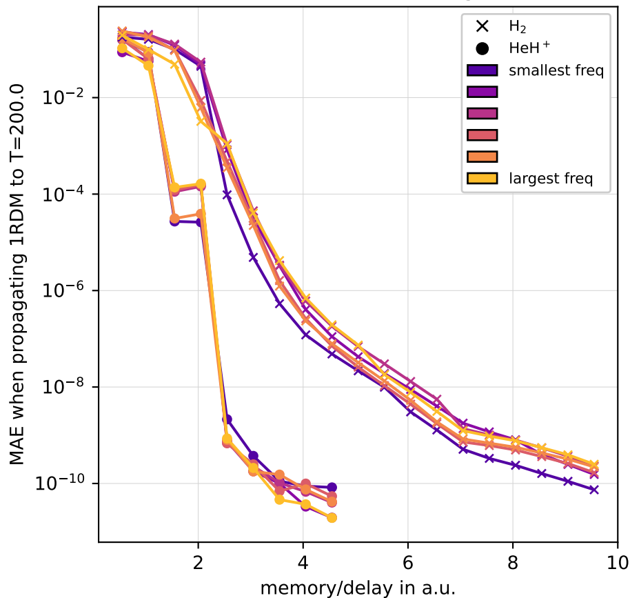
Full CI Field-On 3-21g
