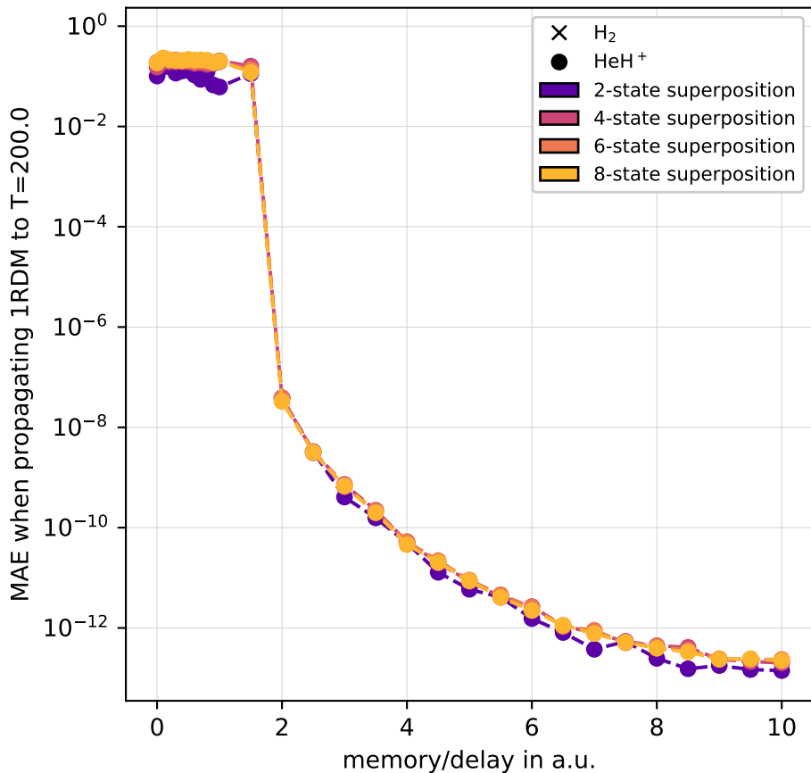
Full CI Field-Off 3-21g
