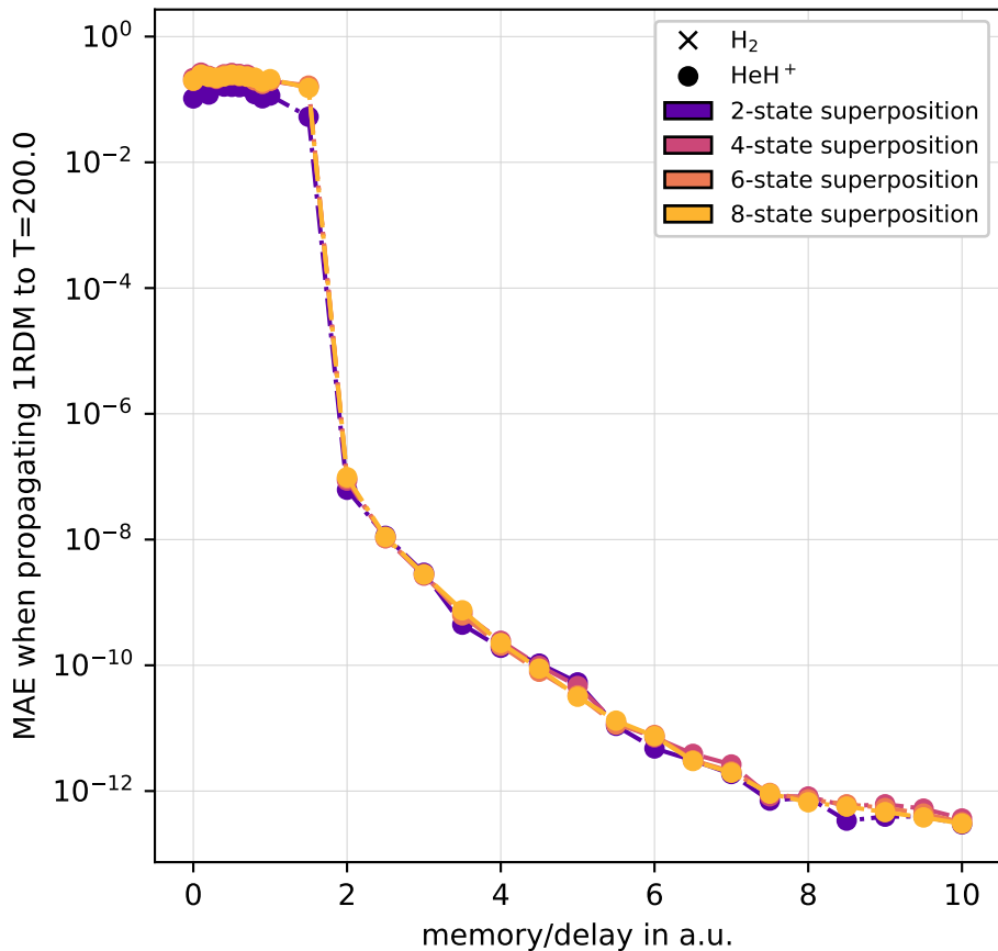
Full CI Field-Off 6-31g
