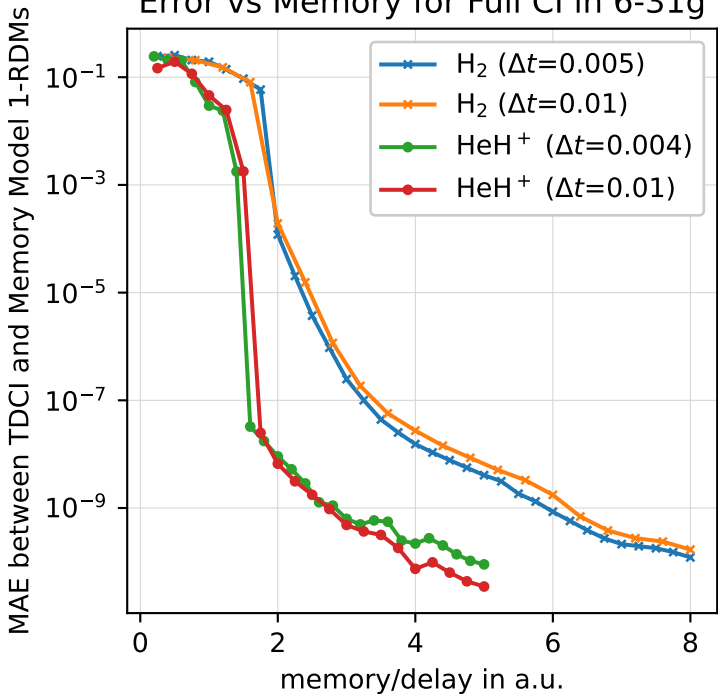
Error vs Memory for Full CI in 6-31g
