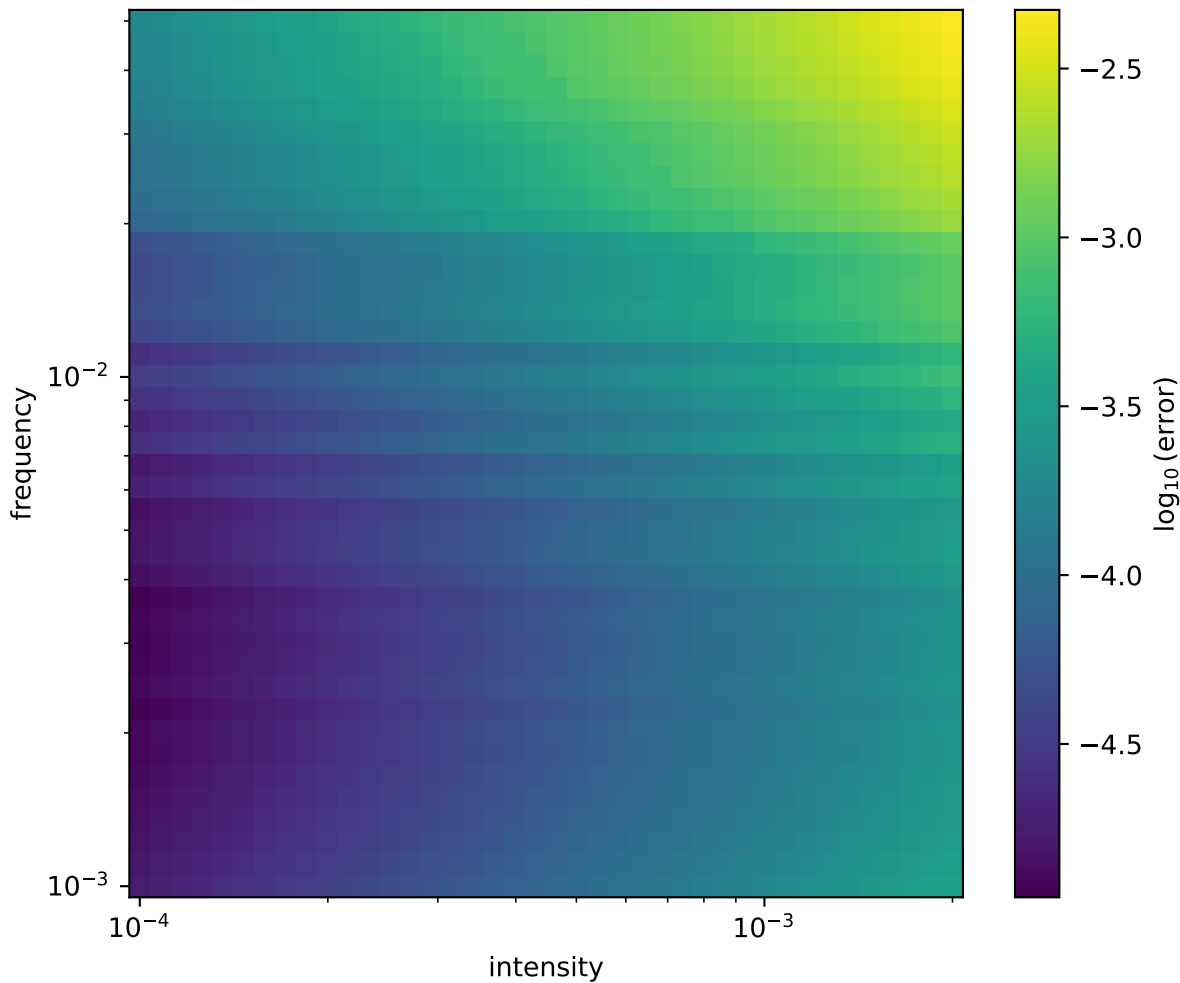
Memory model error for H 2 in 6-31g (field applied for 1 cycle)
