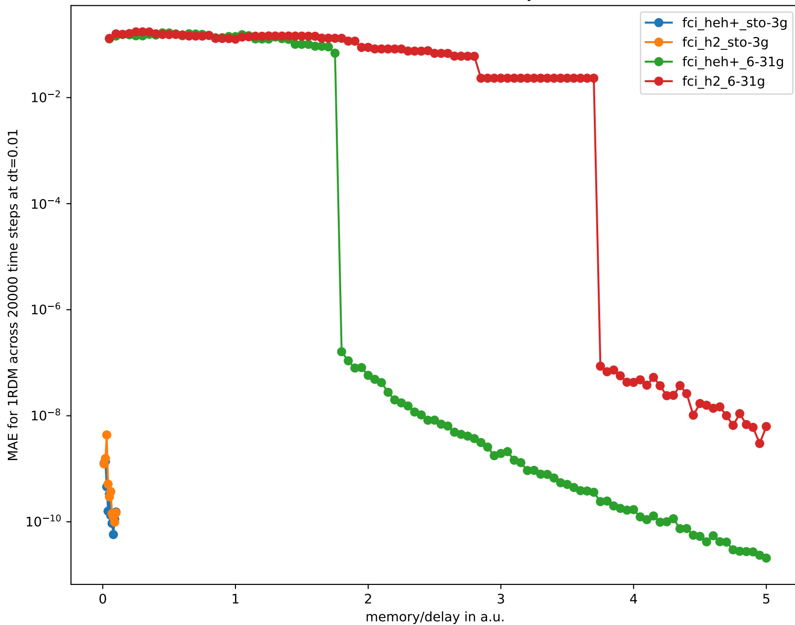
FCI Errors versus Memory
