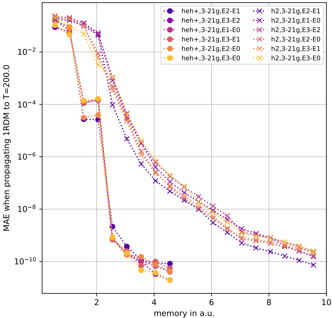
FCI Field-On Results for 3-21g
