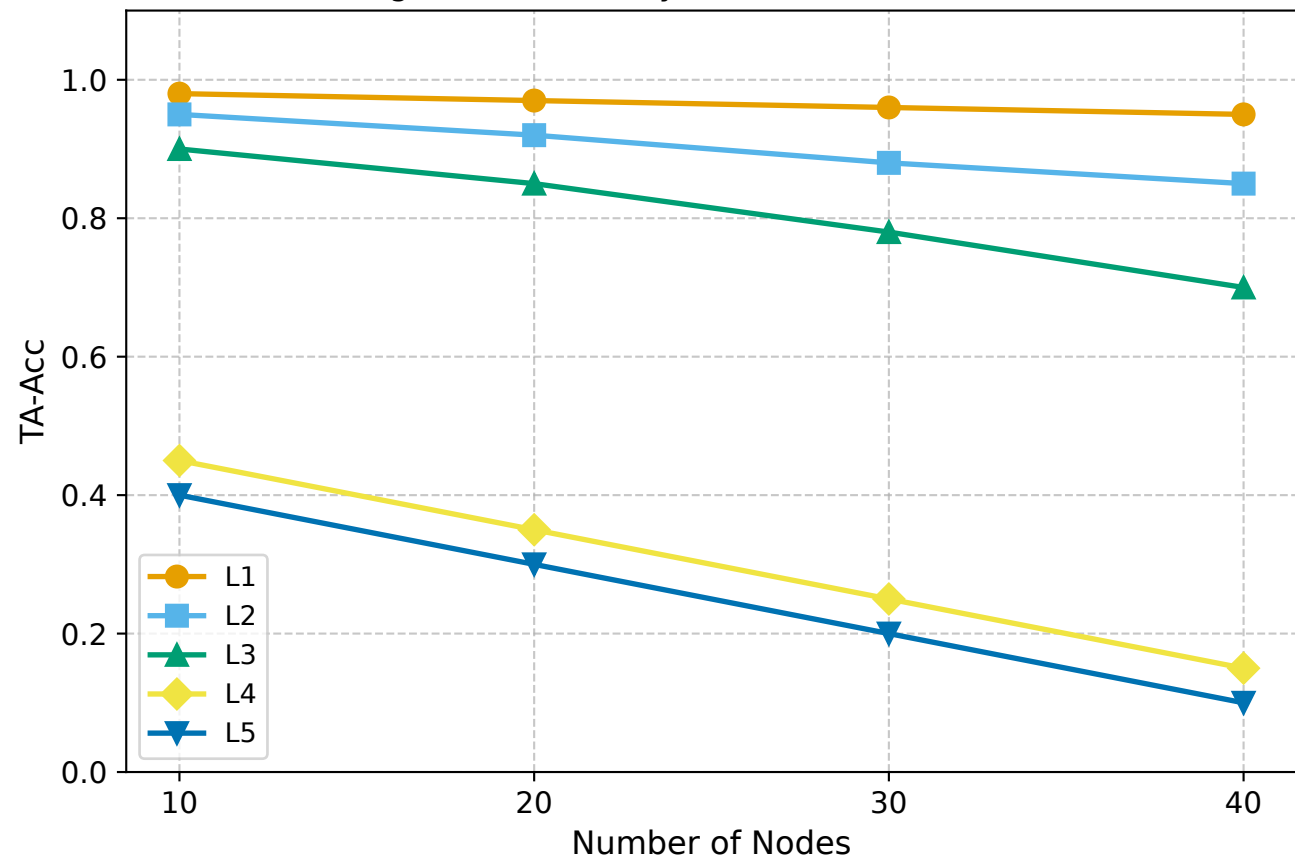
Figure 6: Scalability (Node count vs TA-Acc)
