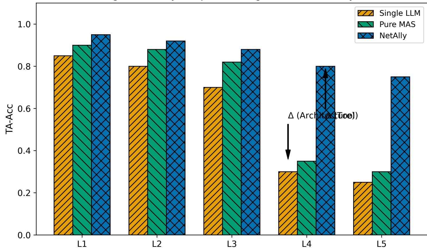
Figure 5: 3-Way Comparison (Single vs MAS vs NetAlly)
