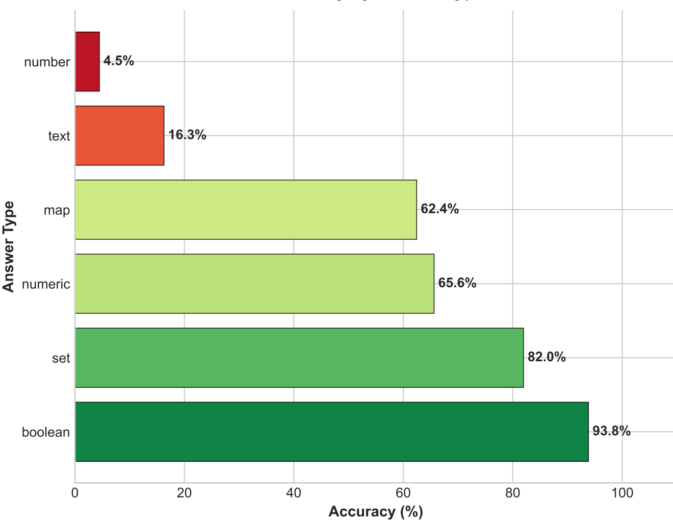
Accuracy by Answer Type
