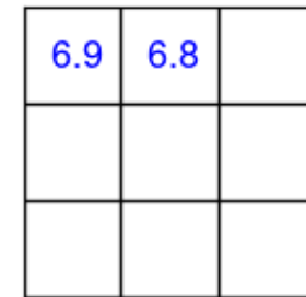
(3, 3, 1)-image convolved
