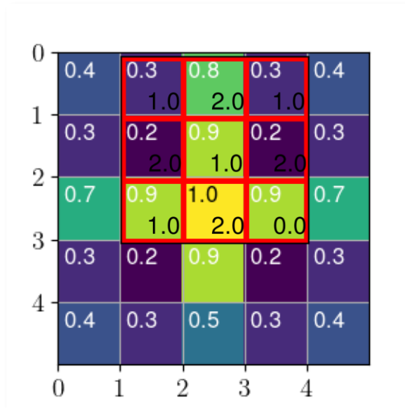
(5, 5, 1)-image
