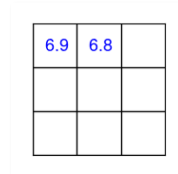
(3, 3, 1)-image convolved
