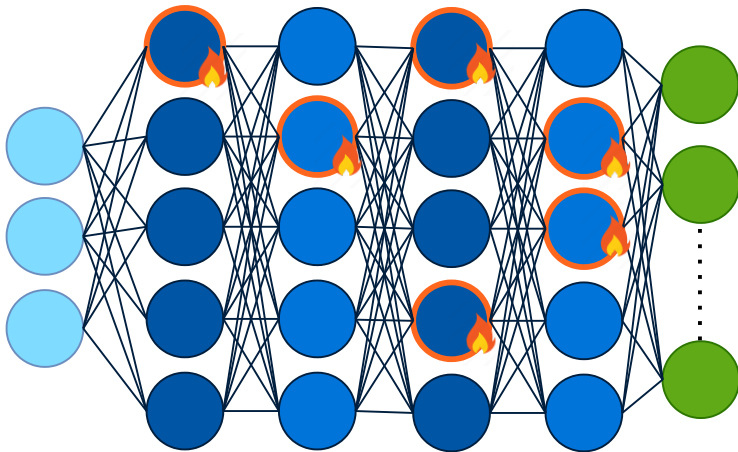
Backdoored model
