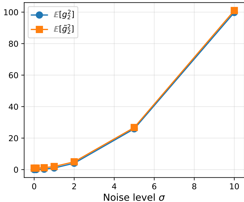
(a) Second moments vs noise
