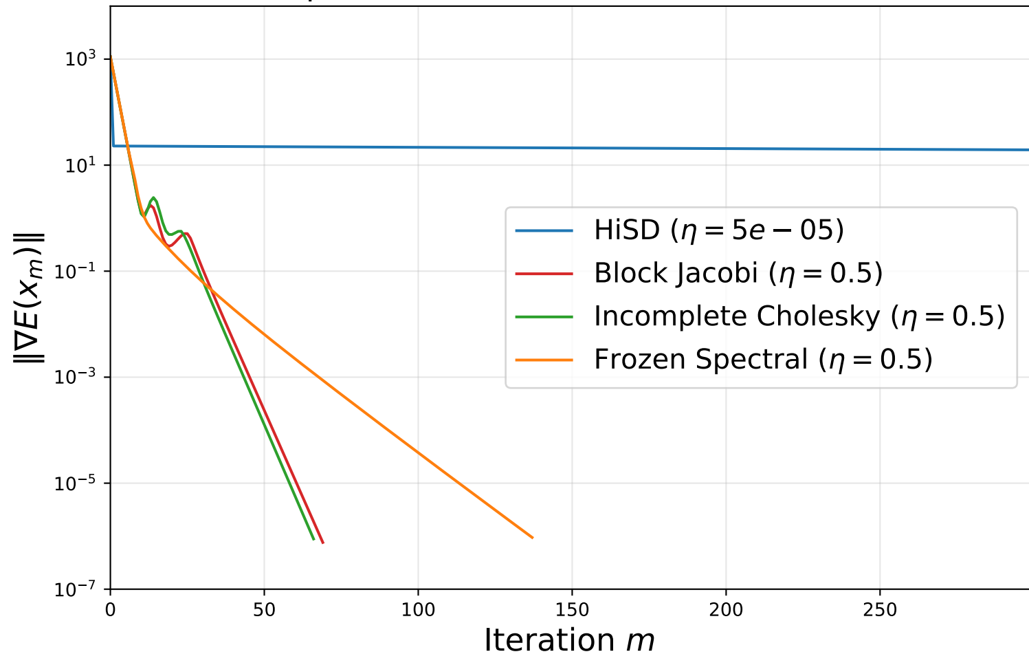
Stiff Coupled Bistable Chain ( N = 50 , K/\delta = 1e + 04 )
