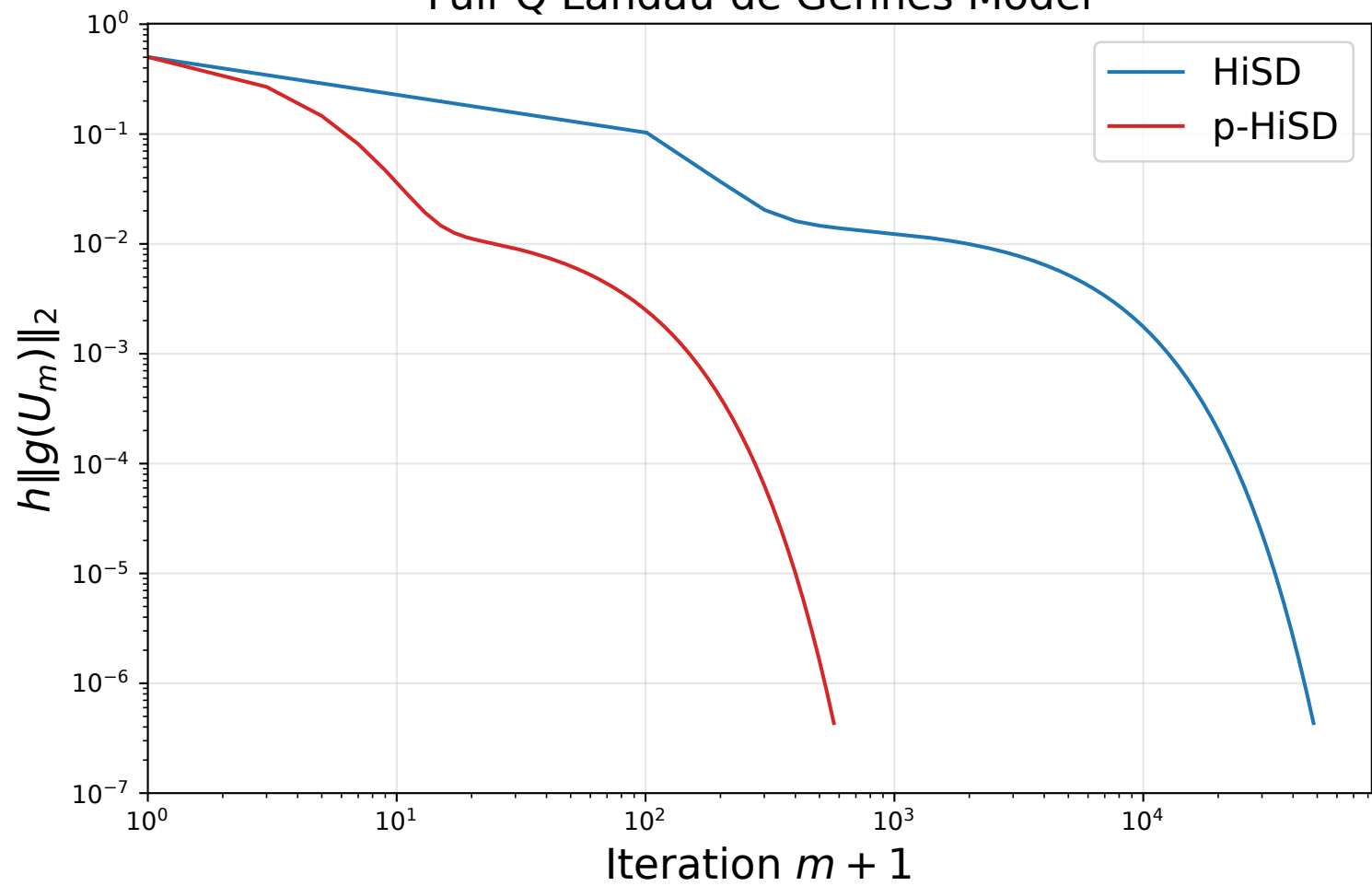
Full-Q Landau-de Gennes Model
