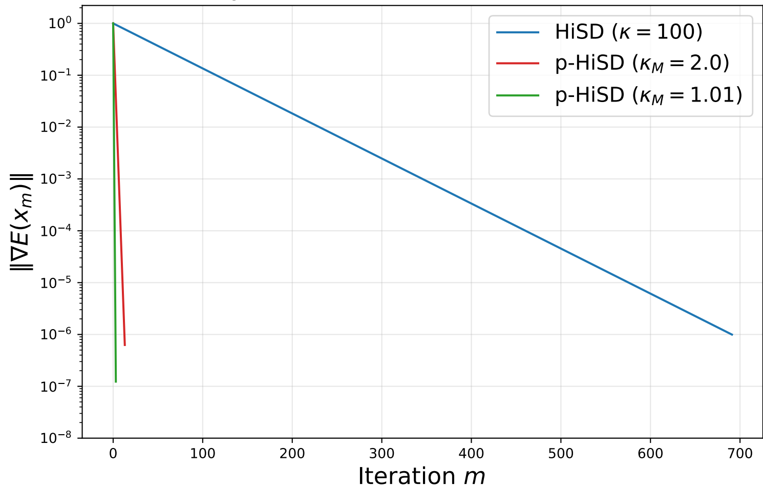
Quadratic Model: Rate Verification
