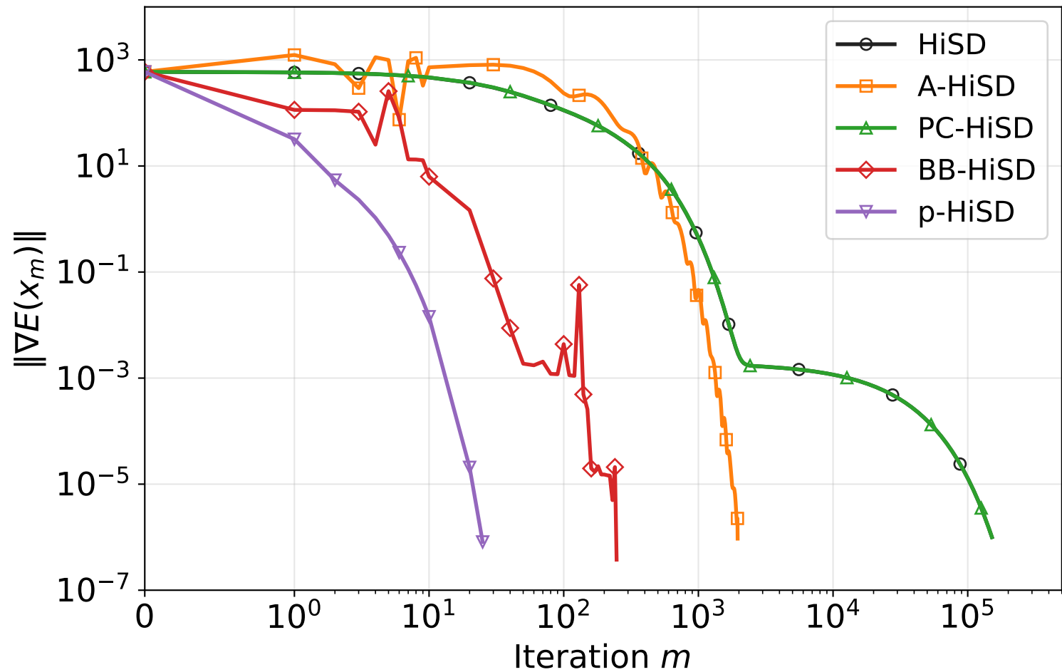
Modified Rosenbrock Function
