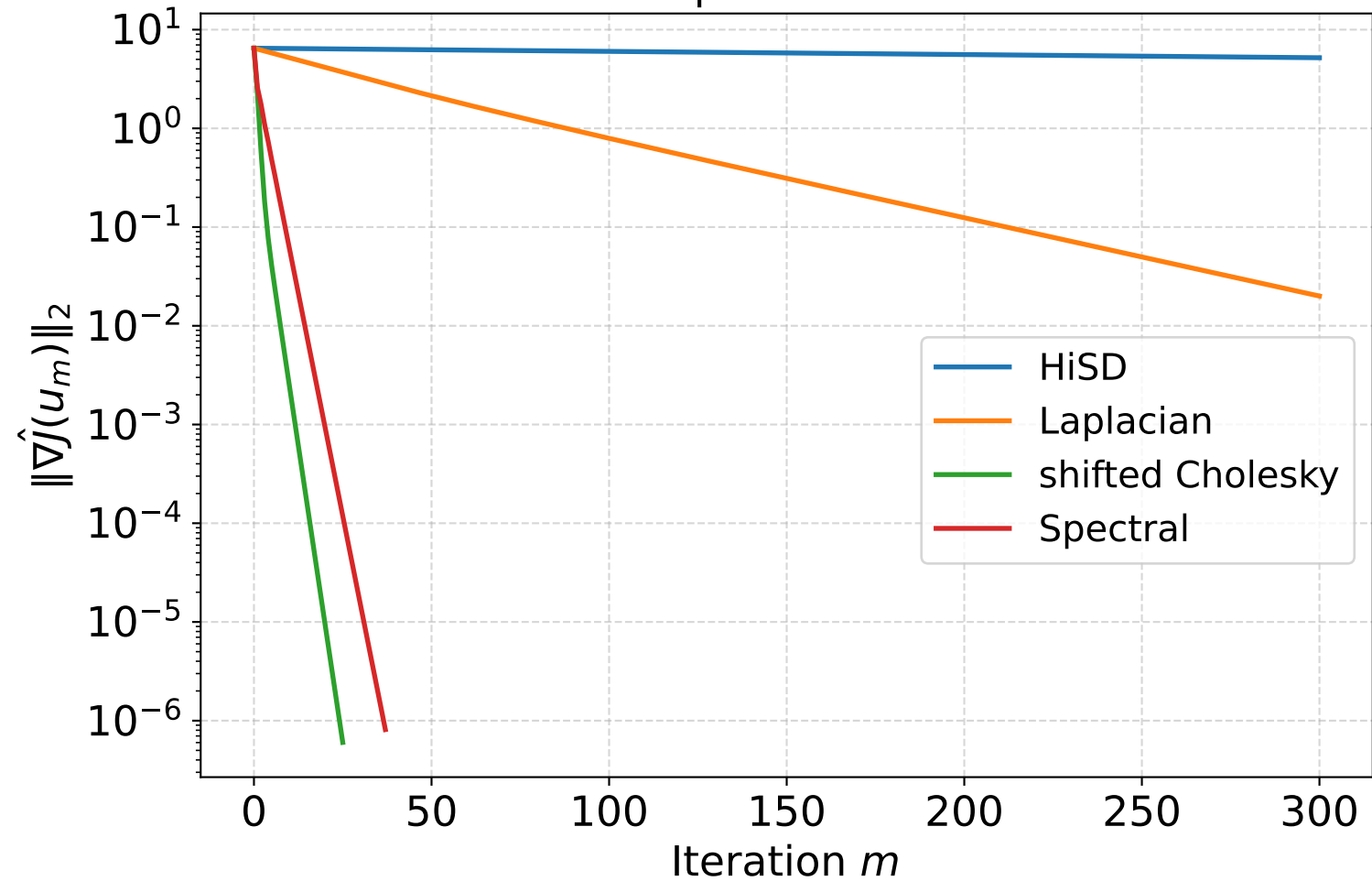
Non-convex Optimal Control Problem
