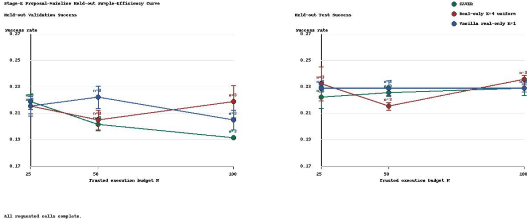
Figure 1: Strict Stage-0 held-out checkpoint curve for N \in \{25, 50, 100\} . Strict CAVR mainly supports backend-data efficiency, while vanilla K = 1 remains a strong raw-success baseline.
