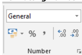
Gambar 23 Formatting Number
