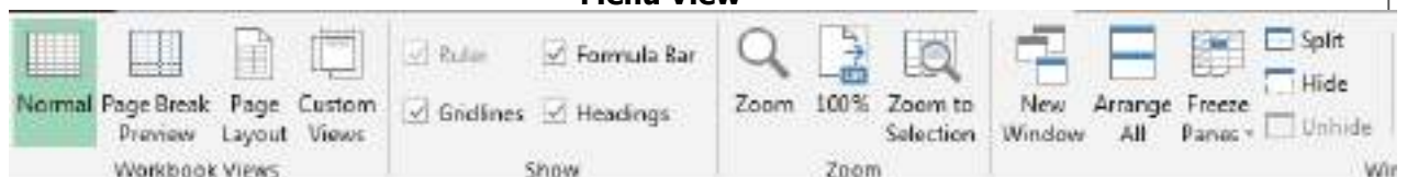
Gambar 30 Menu View
