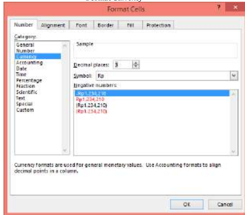
Gambar 42 Format Currency
