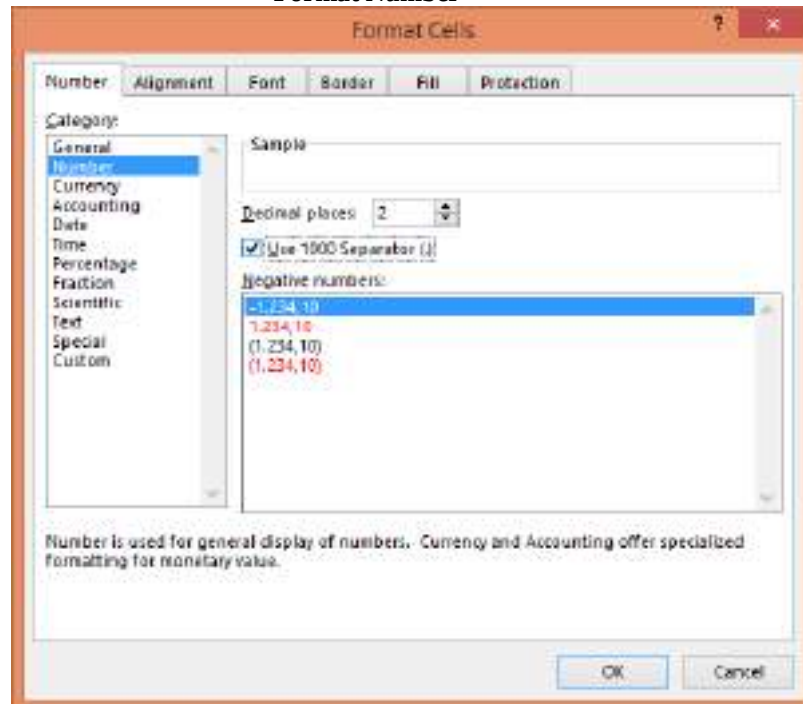
Gambar 41 Format Number
