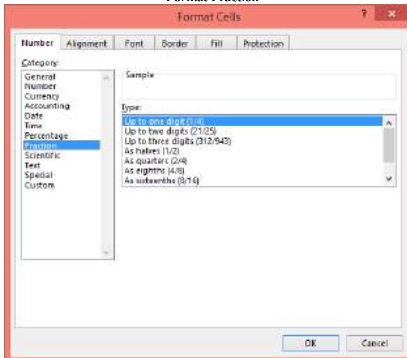
Gambar 44 Format Fraction
