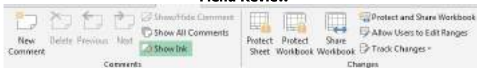
Gambar 29 Menu Review
