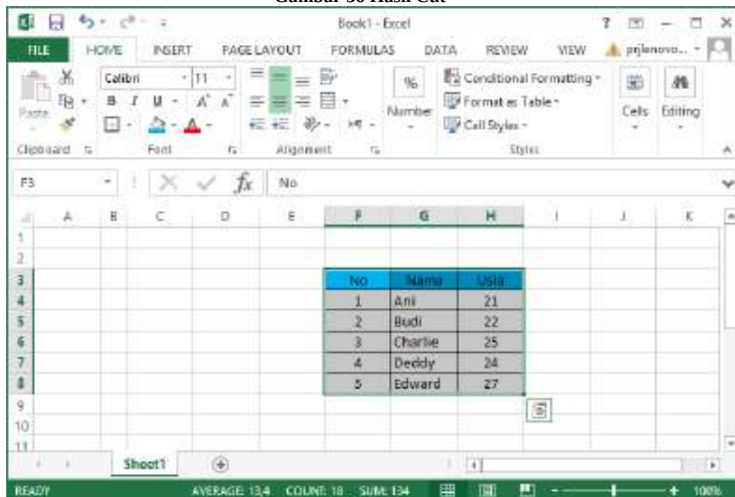
Gambar 56 Hasil Cut
