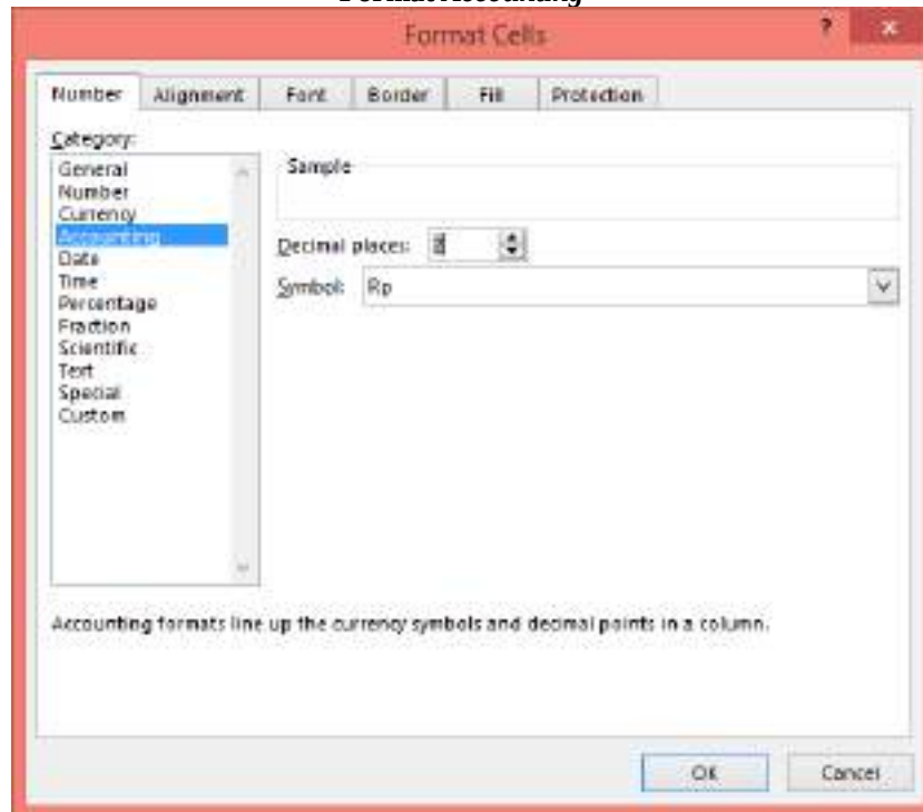
Gambar 43 Format Accounting
