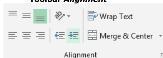
Gambar 22 Toolbar Alignment
