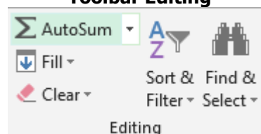
Gambar 25 Toolbar Editing
