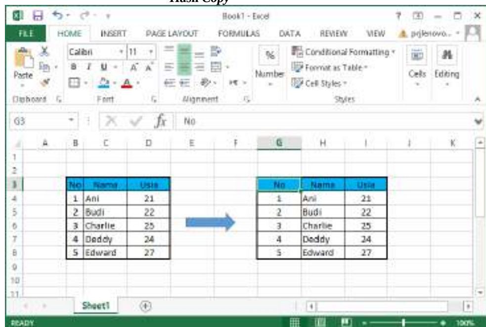
Gambar 55 Hasil Copy
