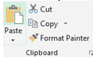
Gambar 20 Toolbar Clipboard
