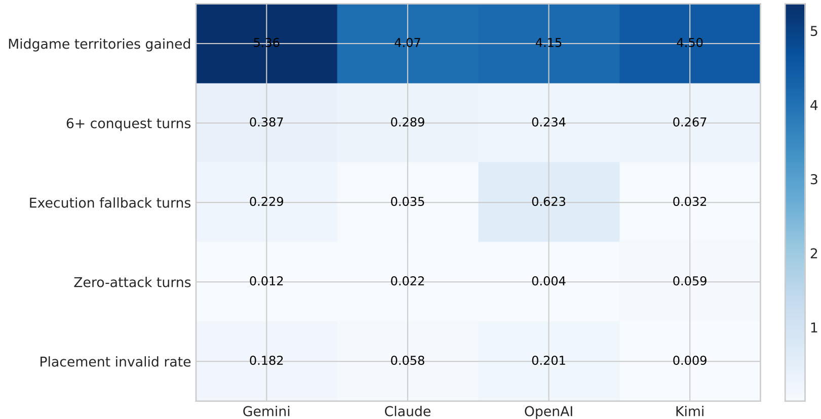
Execution Profile Summary
