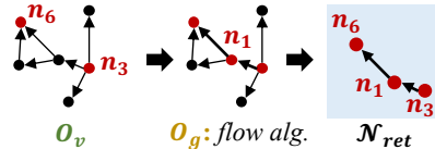
(c) PathRAG ( O_v \rightarrow O_g )
