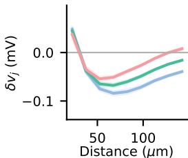
Cotuned, Diffuse
