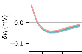
Untuned, Diffuse
