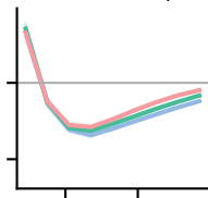
Untuned, Compact
