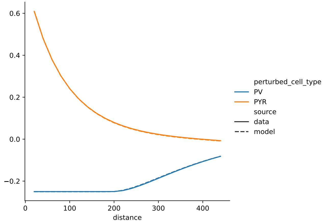
cell_type = PYR
