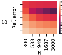
Approx.: 2nd order (naive)
