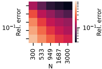
Approx.: 2nd order
