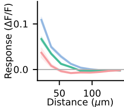
Cotuned, Diffuse
