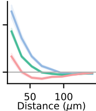
Cotuned, Compact
