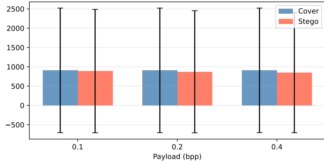
Chi-Square Statistic
