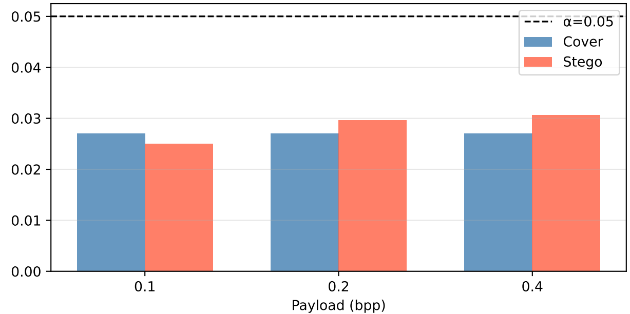
Chi-Square p-value
