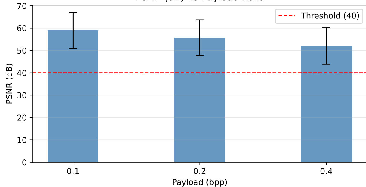
PSNR (dB) vs Payload Rate
