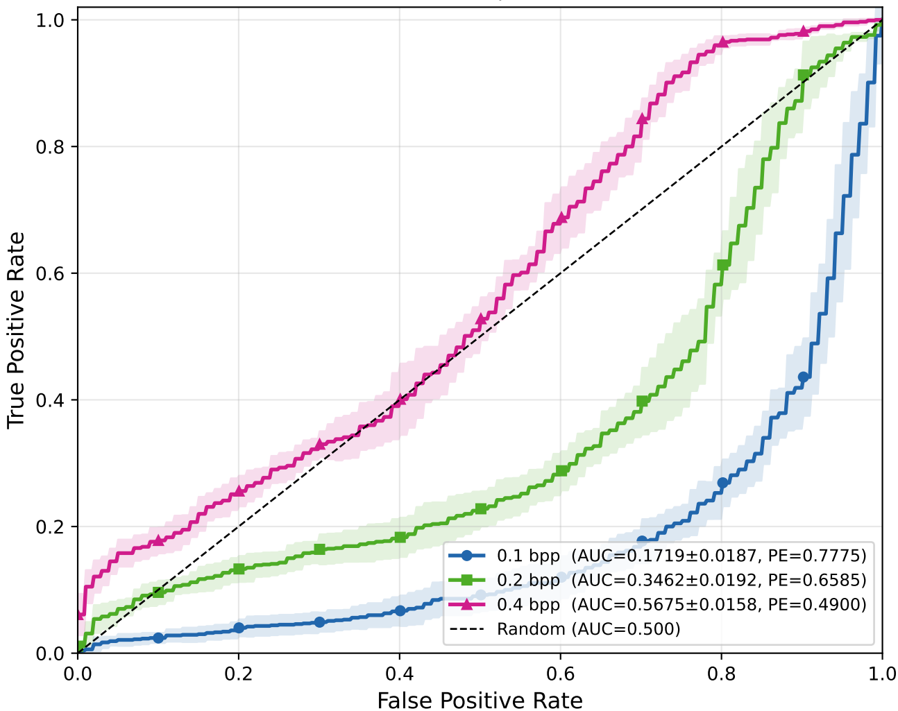
ROC Curves — IWT 3-Channel Steganography SRM+LinearSVC on ALASKA#2 (uncompressed color) (10 trials, 5-fold CV)
